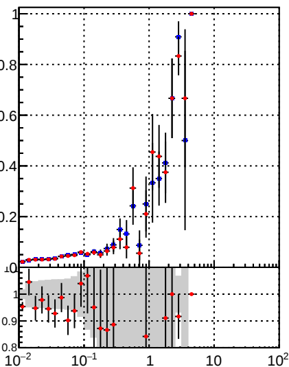
—●— DQM_TT_mkFit-DQM_original —●— DQM_TT_mkFit-DQM_modified3
