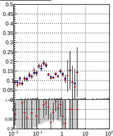
—•— DQM_TT_mkFit-DQM_original —•— DQM_TT_mkFit-DQM_modified3
