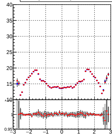
mean hit — DQM_TT_mkFit-DQM_original — DQM_TT_mkFit-DQM_modified3
