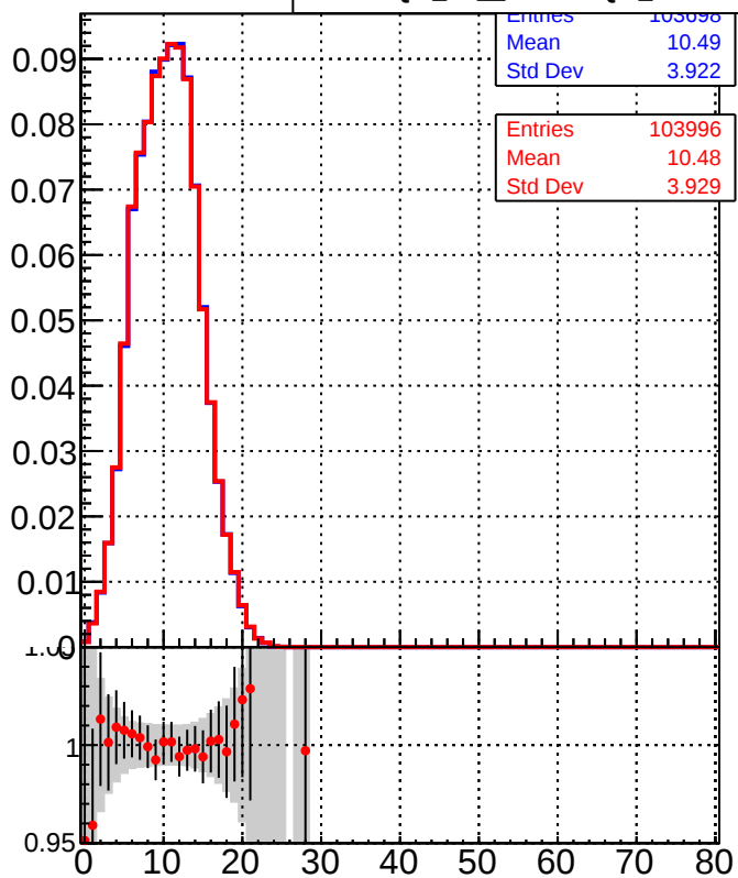
—■— DQM_TT_mkFit-DQM_original —●— DQM_TT_mkFit-DQM_modified3
