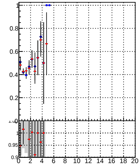
Fake rate vs. DQM_TT_mkFit-DQM_original DQM_TT_mkFit-DQM_modified3
