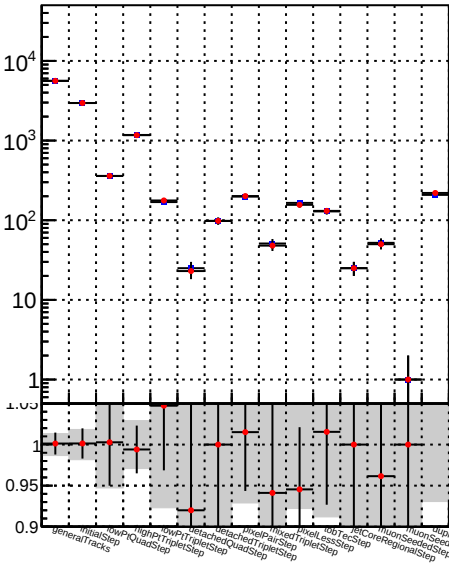
Number —●— DQM_TT_mkFit-DQM_modified3
