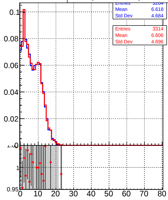
Legend for bottom row: DQM_TT_mkFit-DQM_original (Blue) DQM_TT_mkFit-DQM_modified3 (Red)
