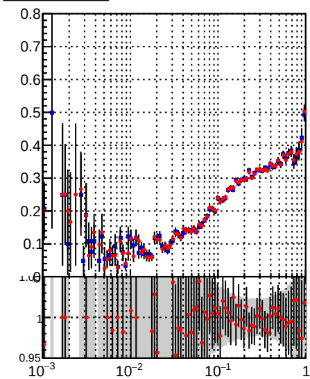
Fake rate vs \sqrt{s} DQM_TT_mkFit-DQM_original DQM_TT_mkFit-DQM_modified3
