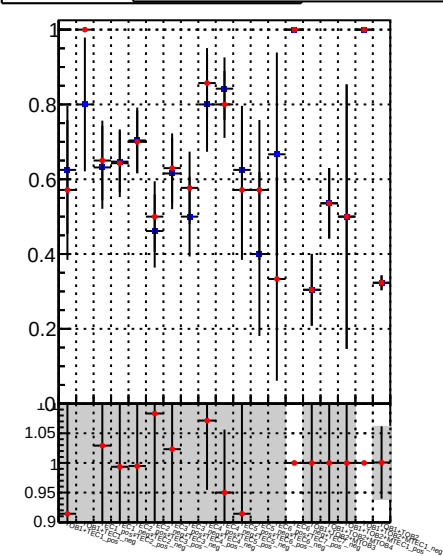
Fake rate vs. DQM_TT_mkFit-DQM_original DQM_TT_mkFit-DQM_modified3
