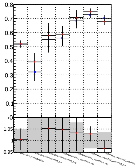
Fake rate vs. DQM_TT_mkFit-DQM_original DQM_TT_mkFit-DQM_modified3
