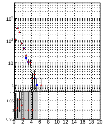
N of reco track vs. \chi^2 —●— DQM TT mkFit-DQM_original —●— DQM TT mkFit-DQM_modified3
