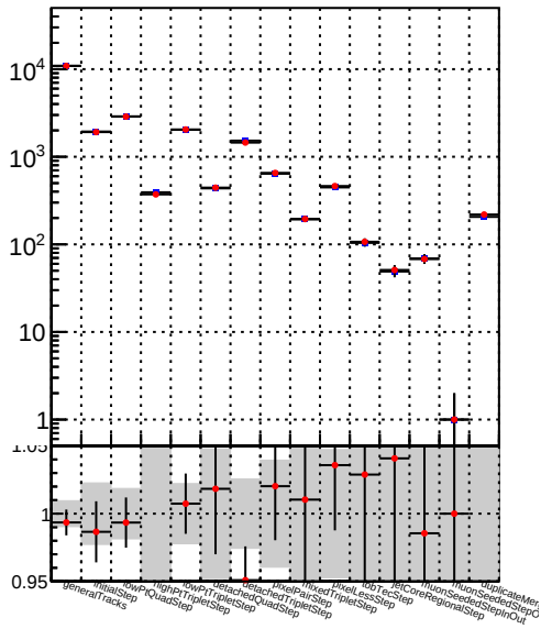
Number —●— DQM_TT__mkFit-DQM_modified3
