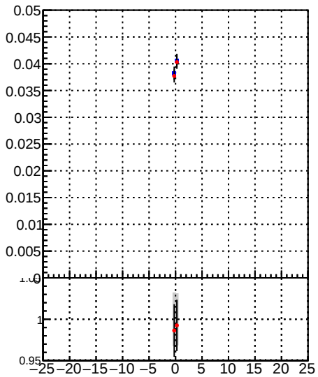
Fake rate vs d —●— DQM_TT_mkFit-DQM_original —●— DQM_TT_mkFit-DQM_modified3
