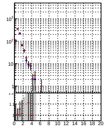
N of reco track vs. \chi^2 vs. \chi^2
