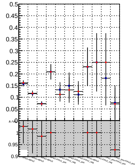
Fake rate vs. DQM_TT_mkFit-DQM_original DQM_TT_mkFit-DQM_modified3
