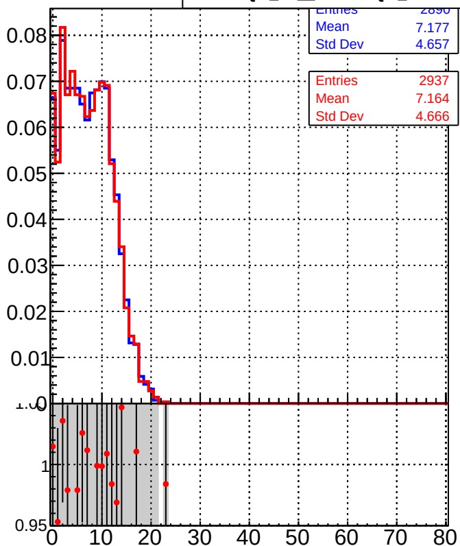
—■— DQM_TT_mkFit-DQM_original —●— DQM_TT_mkFit-DQM_modified3
