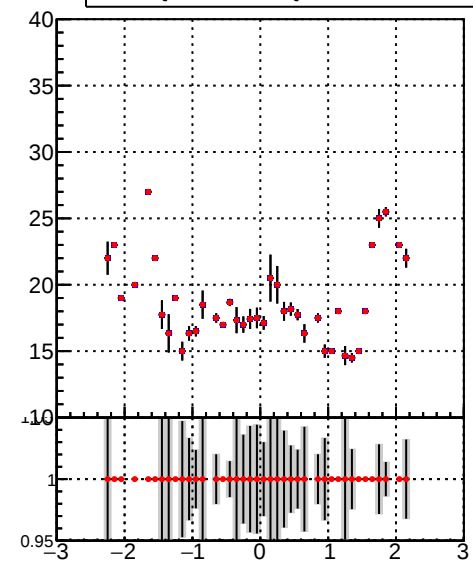
mean hit Legend: DQM_TT_mkFit-DQM_original (blue line with circles), DQM_TT_mkFit-DQM_modified3 (red line with circles)
