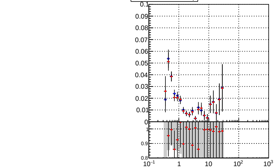
fake+duplicates vs p_T
