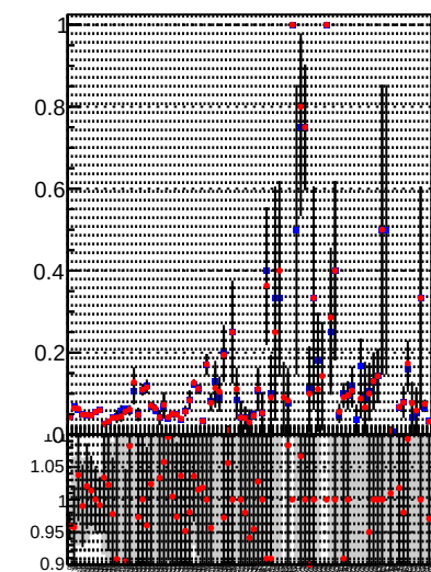
Fake rate vs. —•— DQM TT mkFit-DQM_original —•— DQM TT mkFit-DQM_modified3
