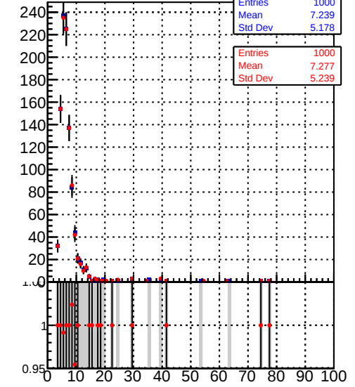
Uncertainty x Coordinate (tagged Vtx) DQM_TT_mkFit-DQM_original DQM_TT_mkFit-DQM_modified3
