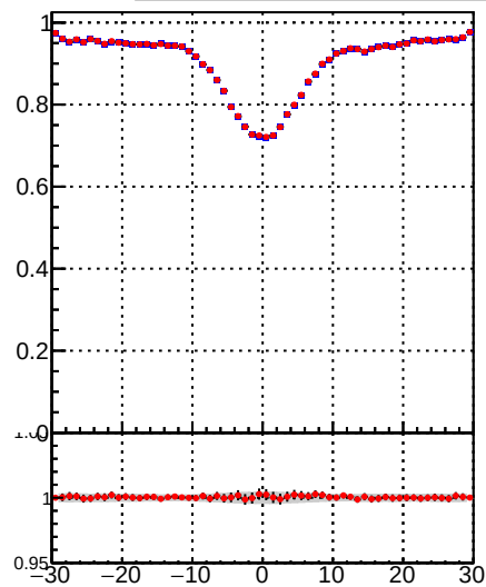
—•— DQM_TT_mkFit-DQM_original —•— DQM_TT_mkFit-DQM_modified3
