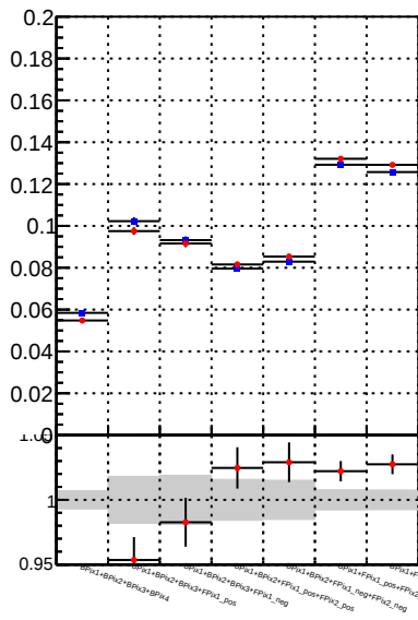
Fake rate vs. —◆— DQM_TT_mkFit-DQM_original —★— DQM_TT_mkFit-DQM_modified3
