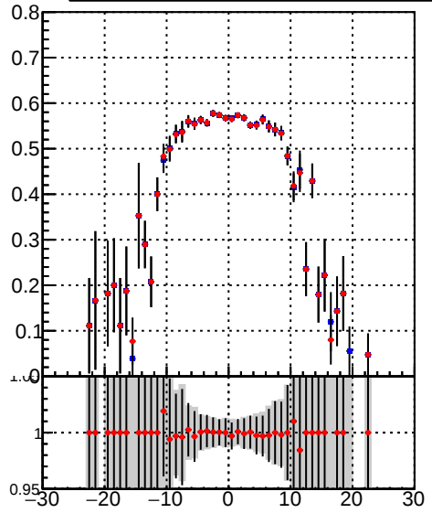
Efficiency vs. sim PV z — DQM_TT_mkFit-DQM_original — DQM_TT_mkFit-DQM_modified3
