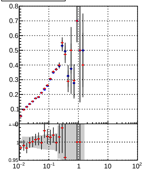
—●— DQM_TT_mkFit-DQM_original —●— DQM_TT_mkFit-DQM_modified3
