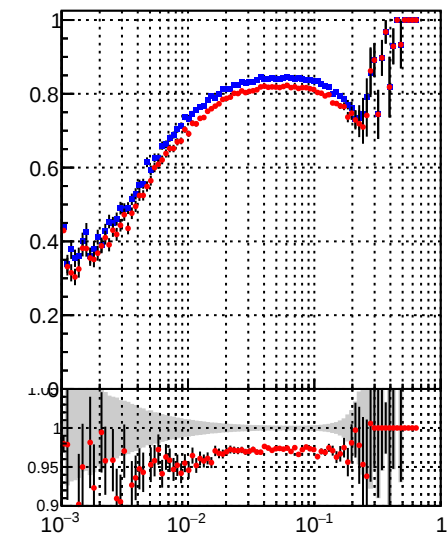
—•— DQM_TT_mkFit-DQM_original —•— DQM_TT_mkFit-DQM_modified3
