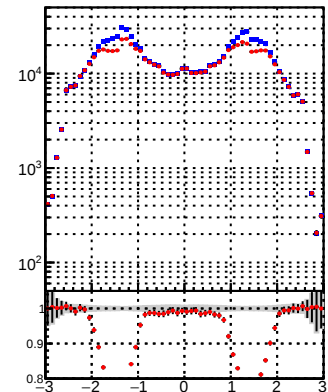
—●— DQM_TT_mkFit-DQM_original —●— DQM_TT_mkFit-DQM_modified3
