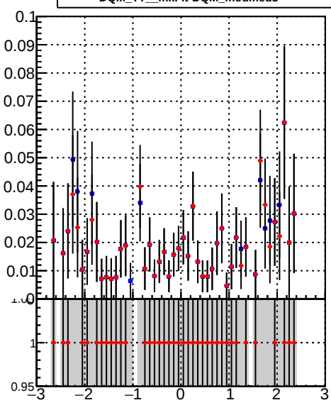
Legend: —●— DQM_TT_mkFit-DQM_original —●— DQM_TT_mkFit-DQM_modified3
