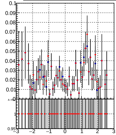
■ DQM_TT_mkFit-DQM_original ■ DQM_TT_mkFit-DQM_modified3
