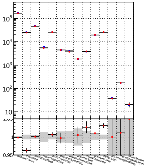
Number —●— DQM_TT__mkFit-DQM_modified3
