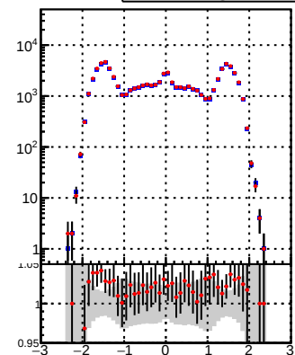
● DQM_TT_mkFit-DQM_original ● DQM_TT_mkFit-DQM_modified3
