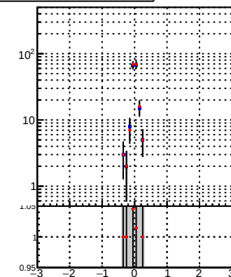
N of associated (recoToSim) tracks vs eta
