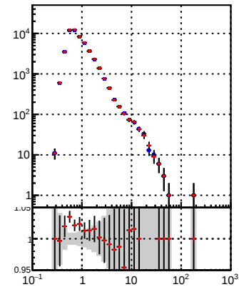
● DQM_TT_mkFit-DQM_original ● DQM_TT_mkFit-DQM_modified3
