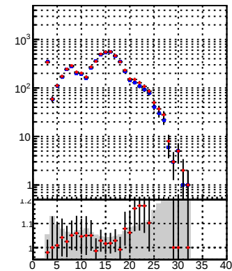
DQM_TT_mkFit-DQM_original DQM_TT_mkFit-DQM_modified3
