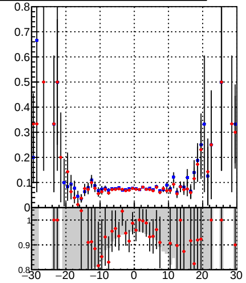
— DQM_TT_mkFit-DQM_original — DQM_TT_mkFit-DQM_modified3 Efficiency vs. sim PV z
