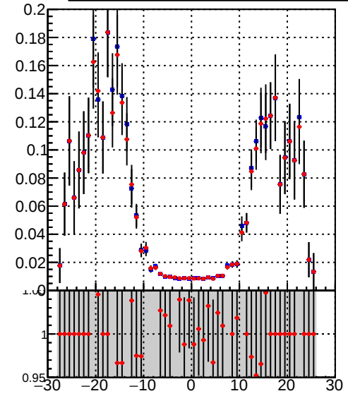
— DQM_TT_mkFit-DQM_original — DQM_TT_mkFit-DQM_modified3 Efficiency vs. sim PV z
