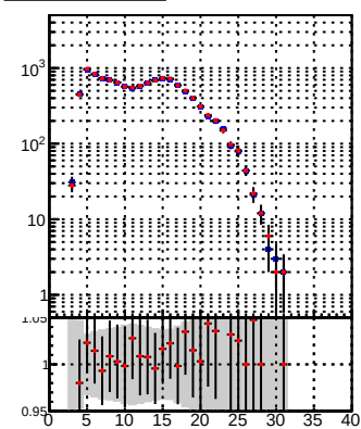
DQM_TT_mkFit-DQM_original DQM_TT_mkFit-DQM_modified3
