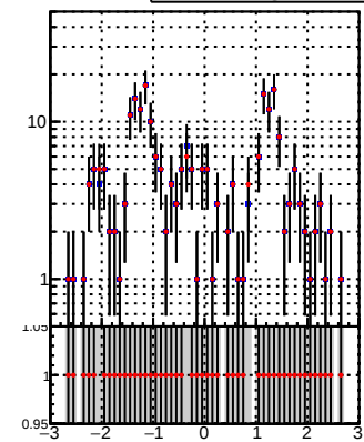
— DQM_TT_mkFit-DQM_original — DQM_TT_mkFit-DQM_modified3
