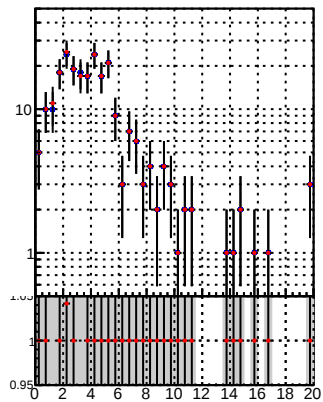
N of reco track vs. \chi^2 for DQM TT and mkFit-DQM variants
