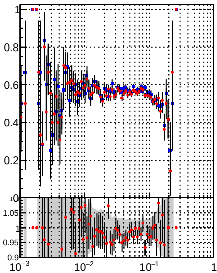
Legend: DQM_TT_mkFit-DQM_original (blue line with markers) DQM_TT_mkFit-DQM_modified3 (red line with markers)
