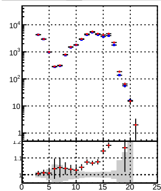
DQM_TT_mkFit-QM_original DQM_TT_mkFit-QM_modified3
