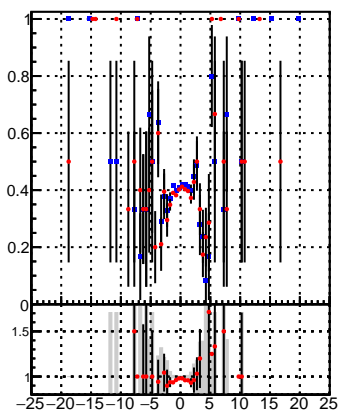
—●— DQM_TT_mkFit-DQM_original —●— DQM_TT_mkFit-DQM_modified3
