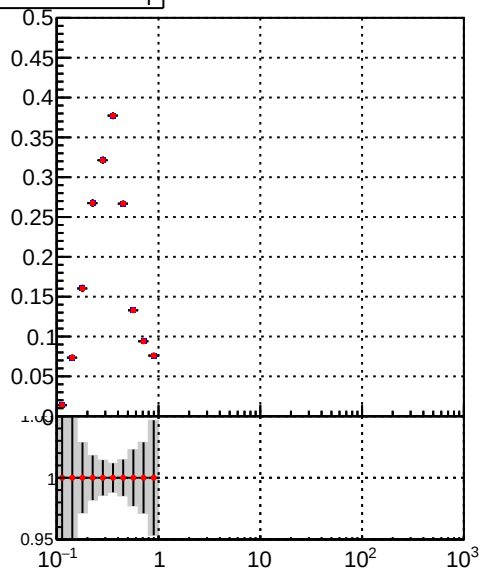
■ DQM_TT_mkFit-DQM_original ◆ DQM_TT_mkFit-DQM_modified2
