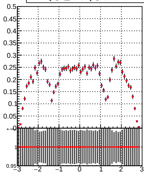
■ DQM_TT_mkFit-DQM_original ◆ DQM_TT_mkFit-DQM_modified2
