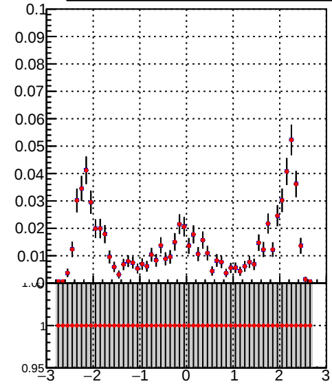
Legend: — DQM_TT_mkFit-DQM_original — DQM_TT_mkFit-DQM_modified2
