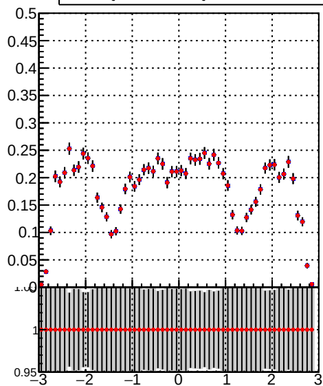
DQM_TT_mkFit-DQM_original DQM_TT_mkFit-DQM_modified2
