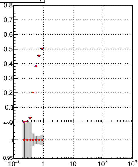
DQM_TT_mkFit-DQM_original DQM_TT_mkFit-DQM_modified2
