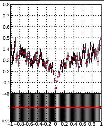
Fake rate vs dz
