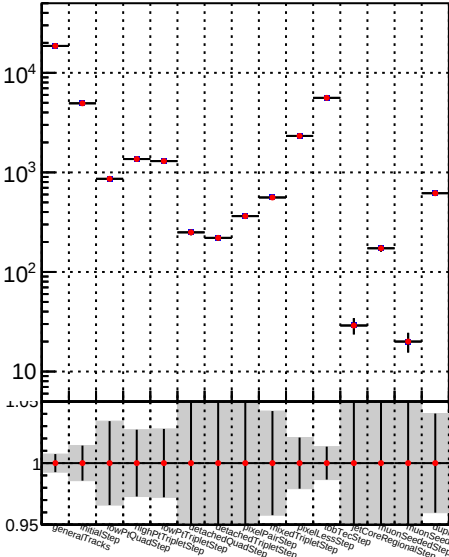
Number —●— DQM_TT__mkFit-DQM_modified2
