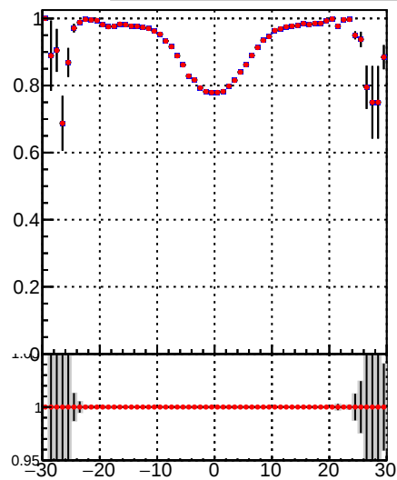
—•— DQM_TT_mkFit-DQM_original —•— DQM_TT_mkFit-DQM_modified2
