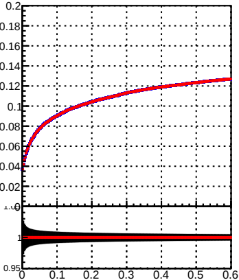
Fake rate
