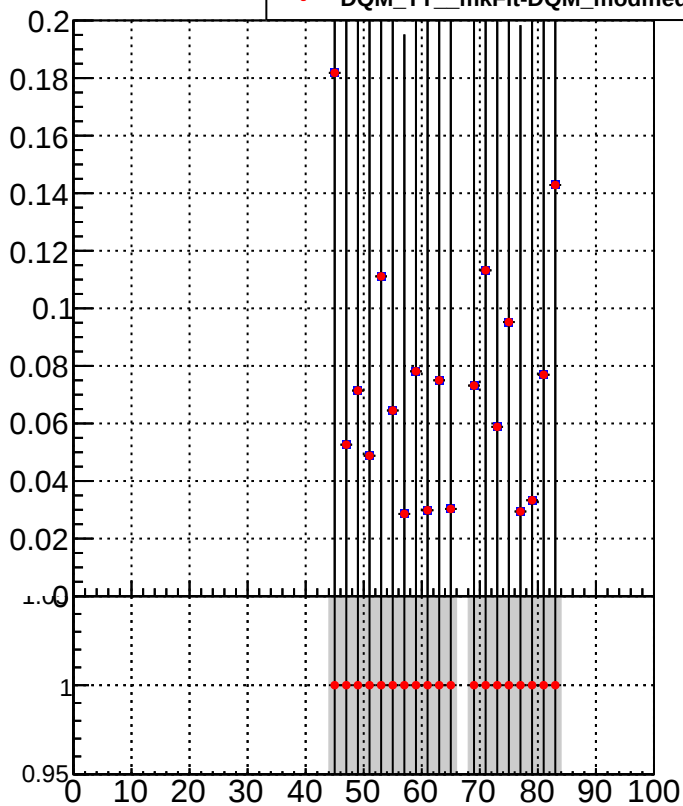
■ DQM_TT_mkFit-DQM_original ● DQM_TT_mkFit-DQM_modified2
