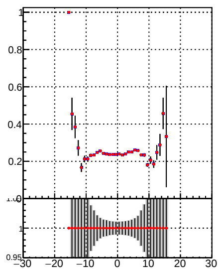
Fake rate vs d —•— DQM_TT_mkFit-DQM_original —•— DQM_TT_mkFit-DQM_modified2
