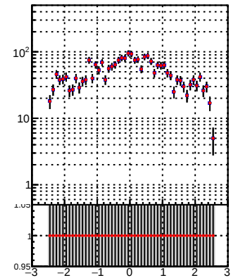
N of reco track vs \eta Legend: \blacksquare DQM_TT_mkFit-DQM_original \bullet DQM_TT_mkFit-DQM_modified2
