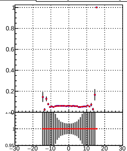
—●— DQM_TT_mkFit-DQM_original —●— DQM_TT_mkFit-DQM_modified2
