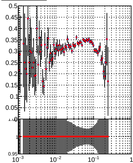
Fake rate vs \sqrt{s} Legend: — DQM_TT_mkFit-DQM_original — DQM_TT_mkFit-DQM_modified2
